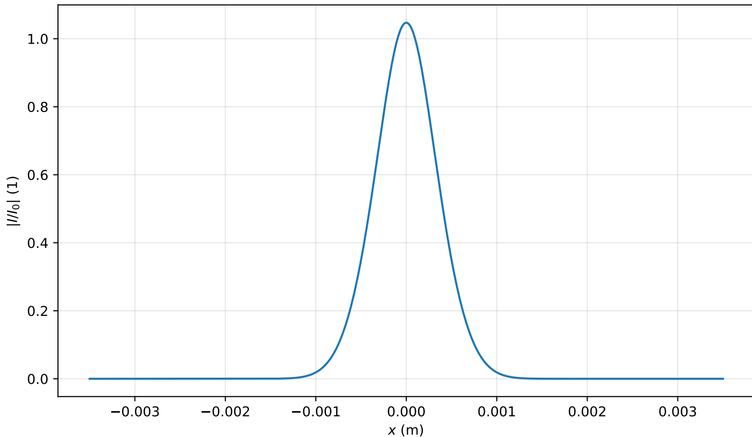
Intensity profile I(x, y = 0, z = 0.398m)/I_0 , P_{in}=0.6P_{cr} , artificial time
